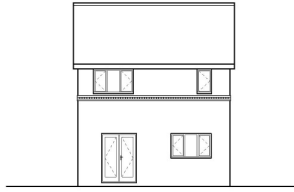
South Elevation.
